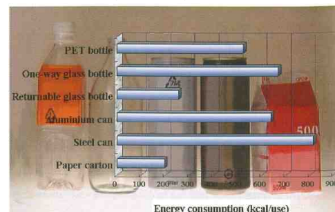
Total energy consumption for life cycle of several kinds of beverage containers
