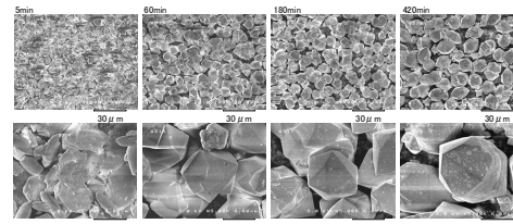
わずか5分の反応でも砒酸鉄結晶が生成 The precipitated sample at 5 minutes confirmed crystals is somewhat irregular. 60分以上の反応時間では数十ミクロンの大型砒酸鉄結晶が生成 The results also showed that large-sized crystal particles formed at 60 min.
