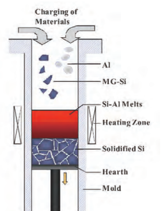
Image of solidification refining process for solar grade Si using Si-Al solvent
